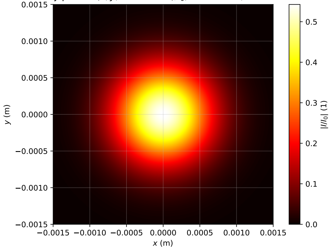
Intensity profile I(x, y, z = 1.990m)/I_0 , P_{in}=0.1P_{cr} , artificial time
